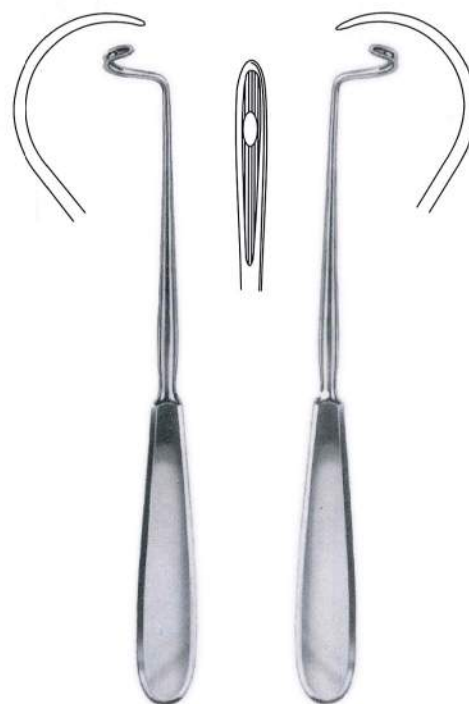
Deschamps Needle
